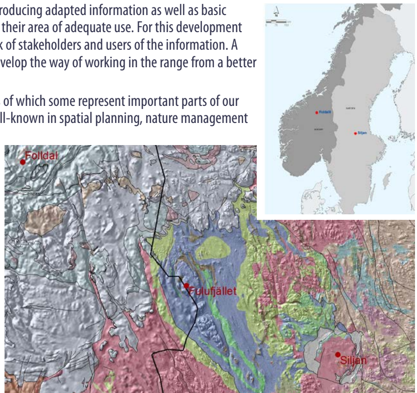
Figure 1 : The Scandinavian peninsula with the case study areas shown as red dots. The main bedrock geological features in the region show that the case study areas complement each other as to the geological character and evolution. From Caledonides (very light blue) in the west, in the middle pre-Cambrian sandstone (blue; very well preserved despite younger Caledonian orogeny), to Precambrian crystalline bedrock (reddish etc.) in the east. A light grey ring of Palaeozoic bedrock shows at Siljan, representing the Siljan ring astrobleme (ca 370 million years old).
